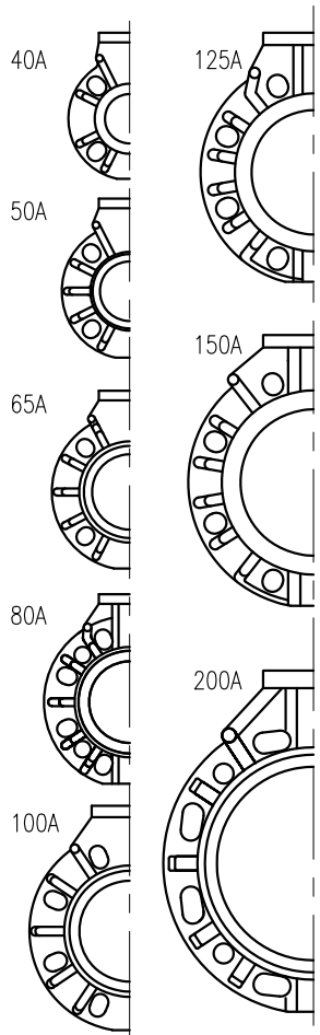
Dimension Table
