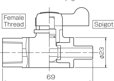
● Female Thread×Spigot
