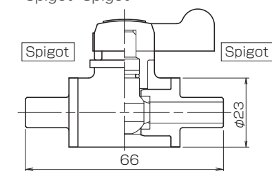
● Spigot×Spigot
