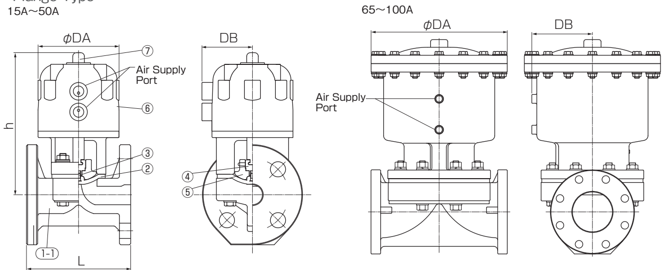
Figure (Flange Type · Socket Type · Thread Type · Butt Type)
