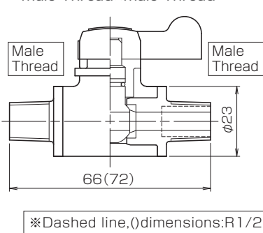
● Male Thread×Male Thread
