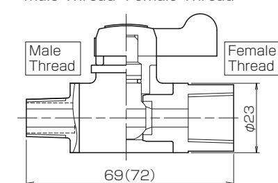
● Male Thread×Female Thread
