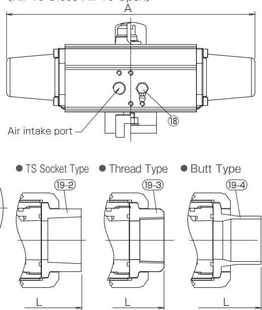
Figure (Flange Type · TS Socket Type · Thread Type · Butt Type)
