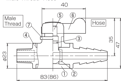
● Male Thread×Hose
