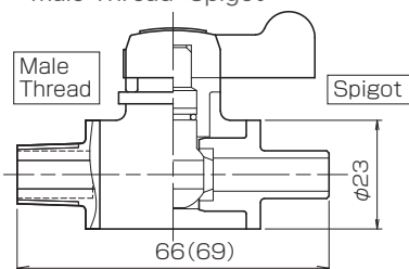
● Male Thread×Spigot
