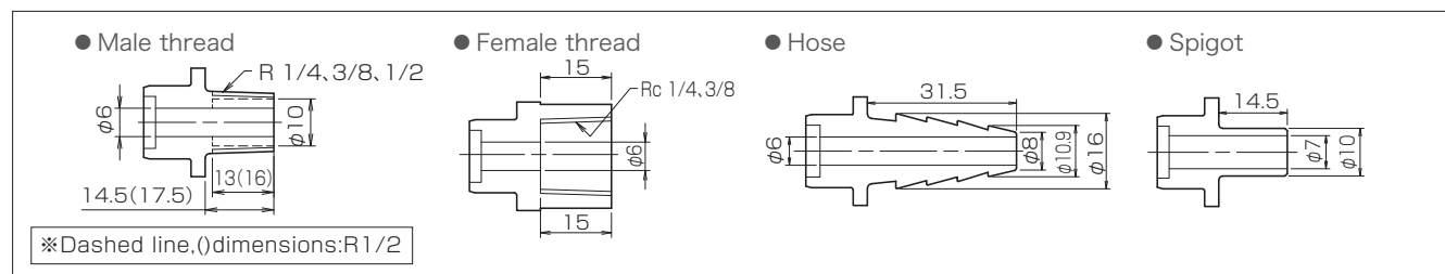
● Male Thread×Hose
