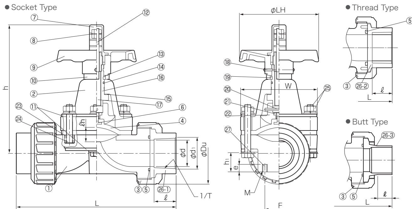
Figure (Socket Type · Thread Type · Butt Type)
