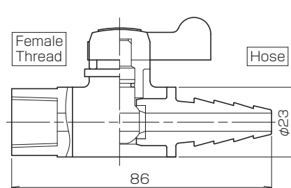
● Female Thread×Hose
