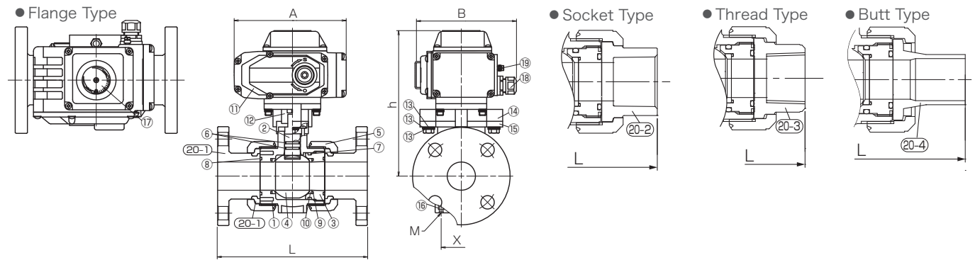
Figure (Flange Type · Socket Type · Thread Type · Butt Type)
