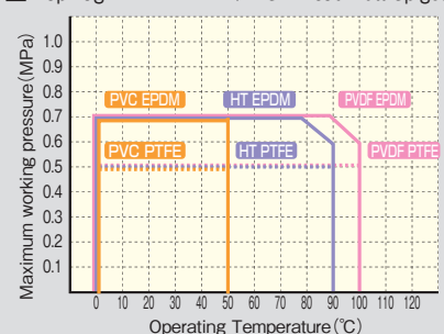
■ Diaphragm:EPDM-PTFE/TS-Thread-Butt Spigot
