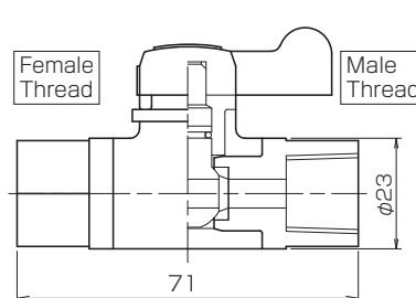
● Female Thread×Female Thread
